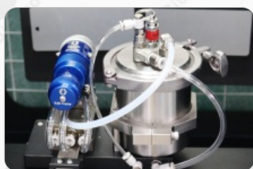
Spray gun
